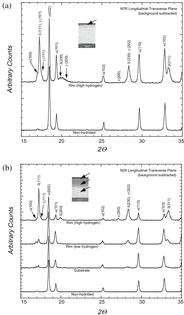
Fig. 8. Diffraction patterns from the L–T plane of cladding with hydride-rim thicknesses (radial-average hydrogen content) of (a) \approx 40 \mu\text{m} ( \approx 400 wt ppm) (Westinghouse cladding) and (b) \approx 260 \mu\text{m} ( \approx 2000 wt ppm) (Sandvik cladding); arrows in inset micrographs show depths after polishing from where patterns were taken. Non-hydrided patterns are also shown for comparison.
