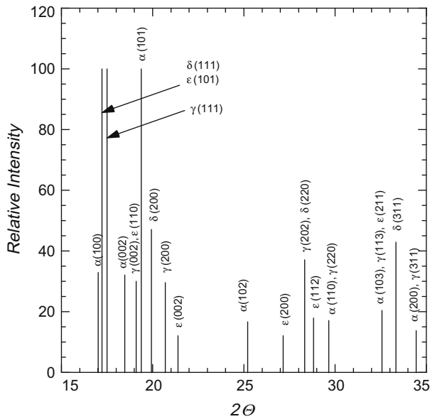
Fig. 4. X-ray diffraction peaks based on data from powder diffraction files for α-Zr, γ-ZrH x (x ≈ 1), δ-ZrH x (x ≈ 1.66), and ε-ZrH x (x ≈ 2) for beam energy of 15 keV; note, for α-Zr, (hkl) is reduced to (hkl) by assuming h + k = -i.
